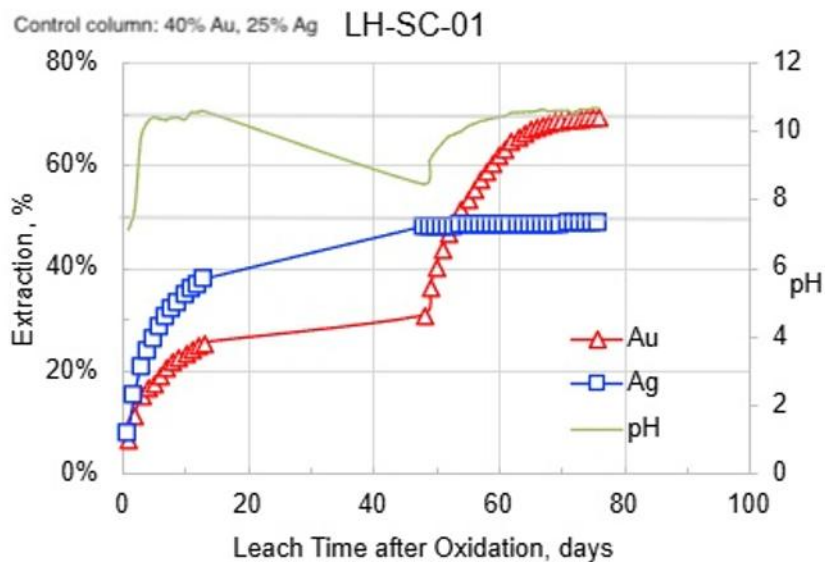
Figure 13-4. BaseMet Pre-Oxidation Column Leach Test for the Santa Fe Sulfide Deposit BaseMet [2026]
