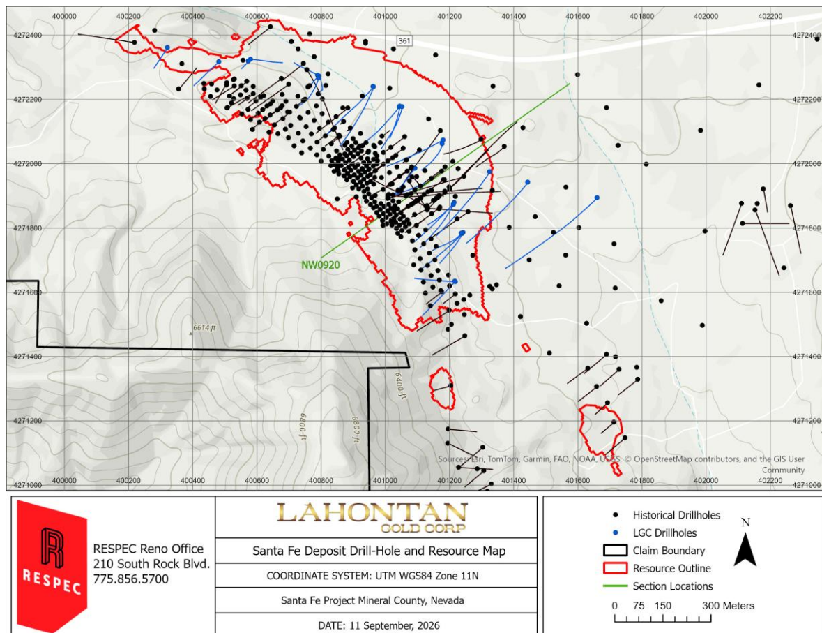
Figure 14-1. Santa Fe Deposit Drill-Hole Map with Mineral Resource Outline
