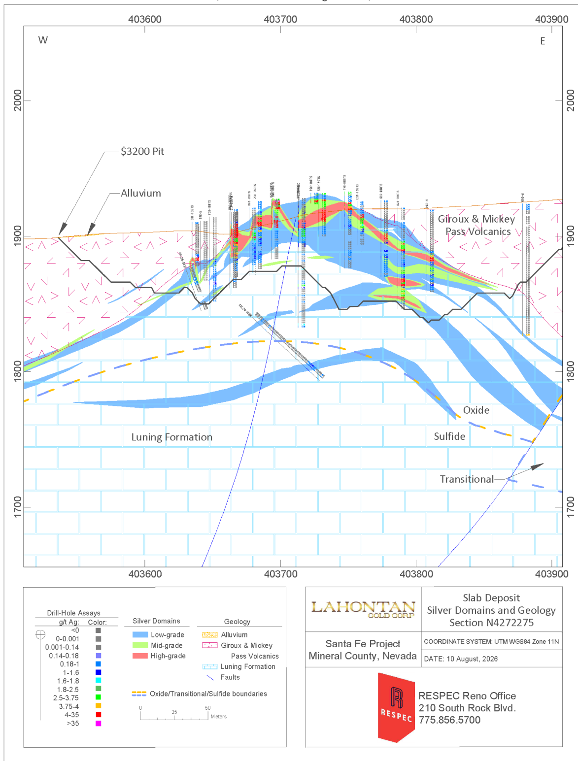
Figure 14-9. Slab Deposit Silver Domains and Geology—Section N4272275
