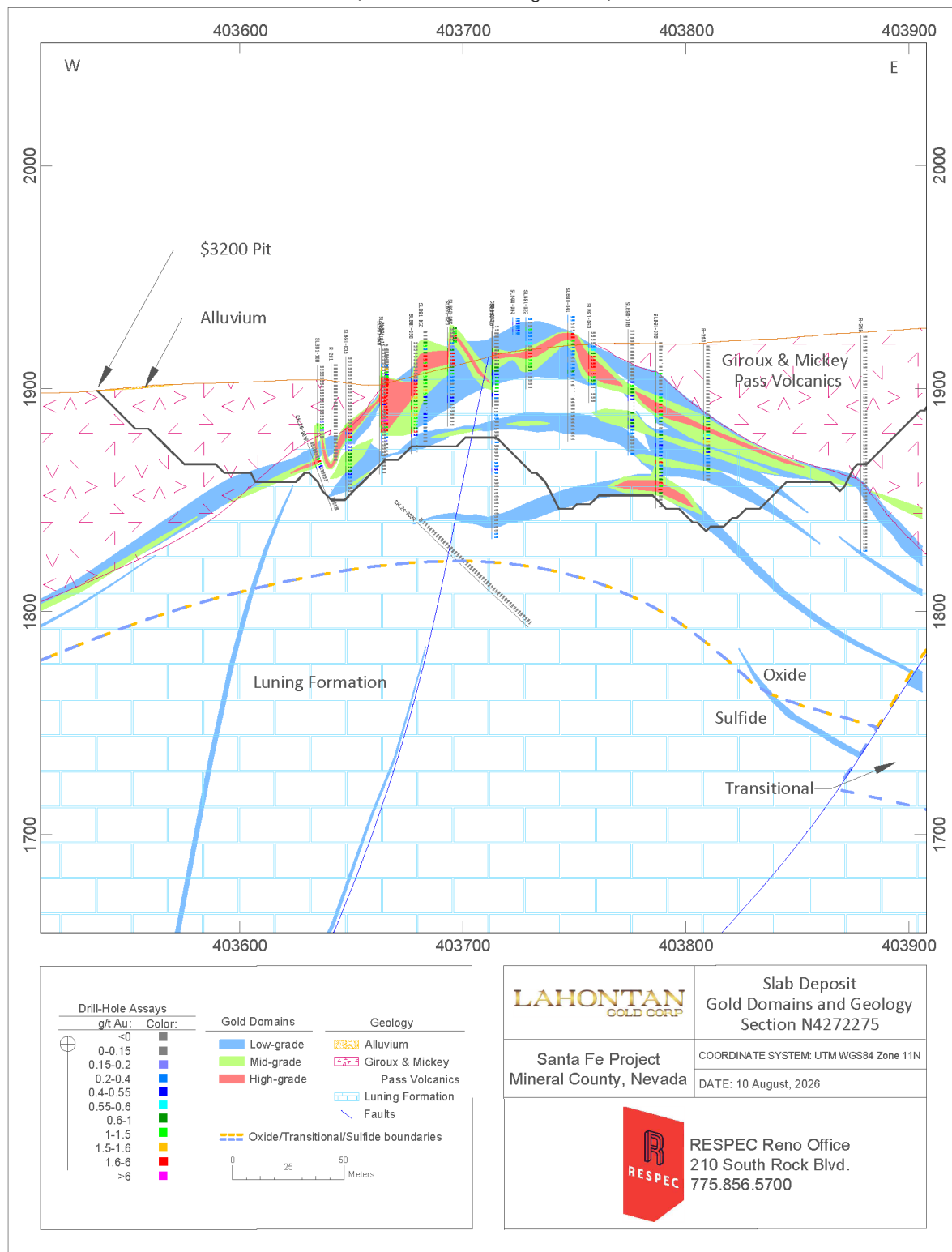
Figure 14-4. Slab Deposit Gold Domains and Geology – Section N4272275
