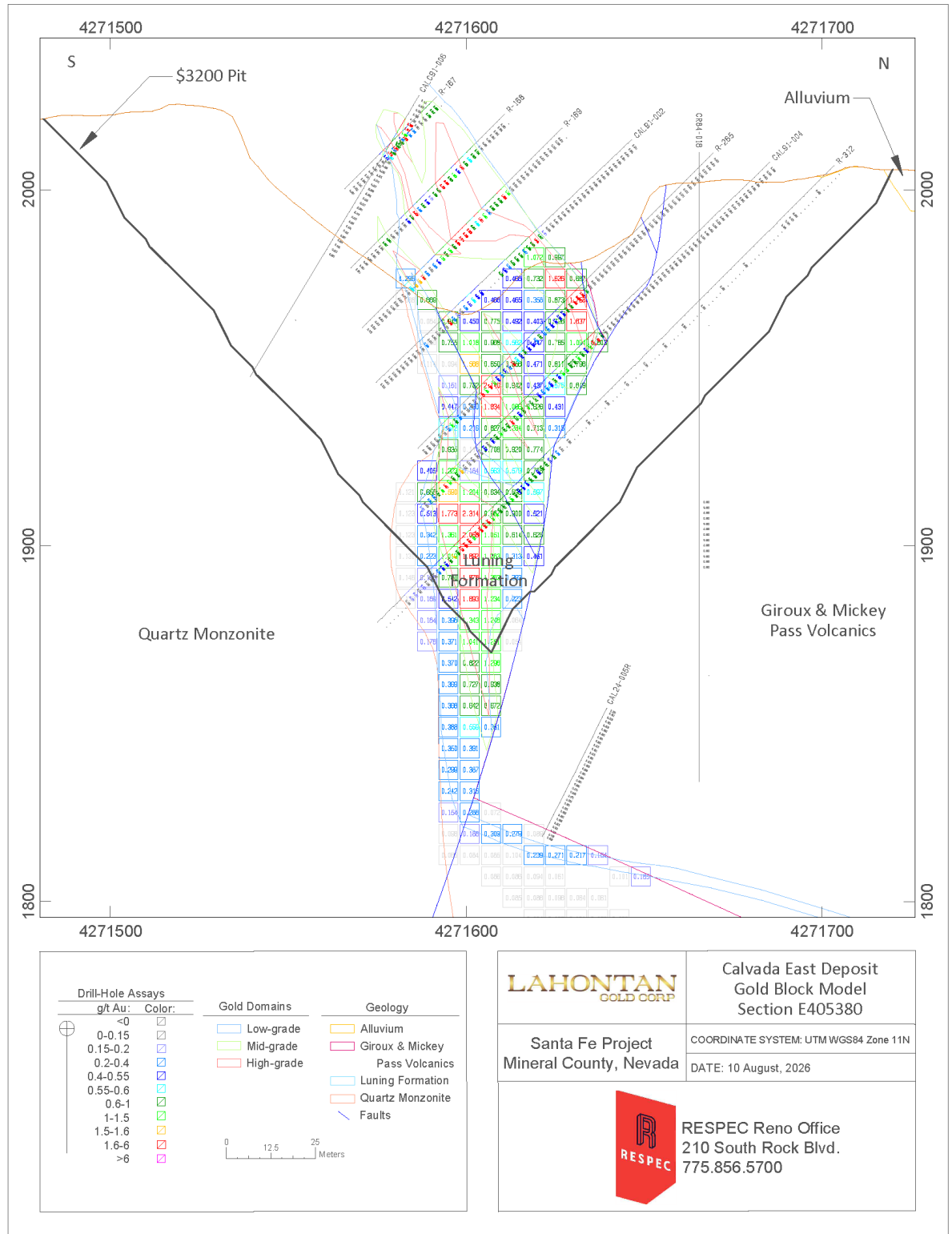
Figure 14-16. Calvada East Deposit Gold Domains and Block Model – Section E405380
