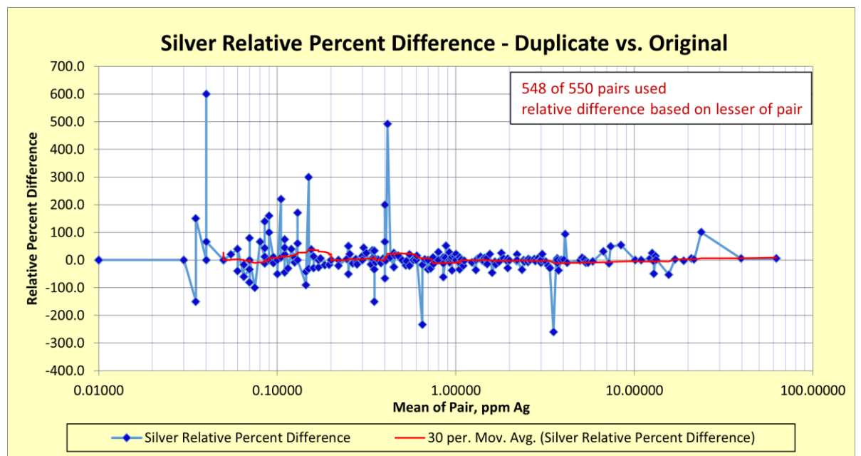
Figure 11-7. Relative Percent Difference Plot of Silver Field Duplicates
