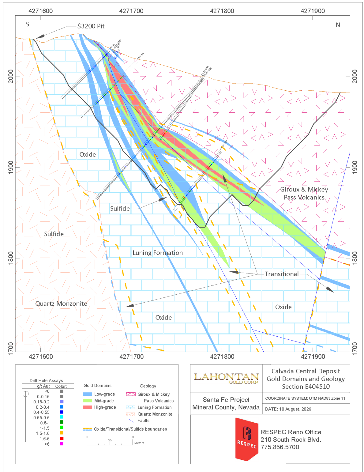
Figure 14-5. Calvada Central Deposit Gold Domains and Geology – Section E404510 (Section location on Figure 14-2)
