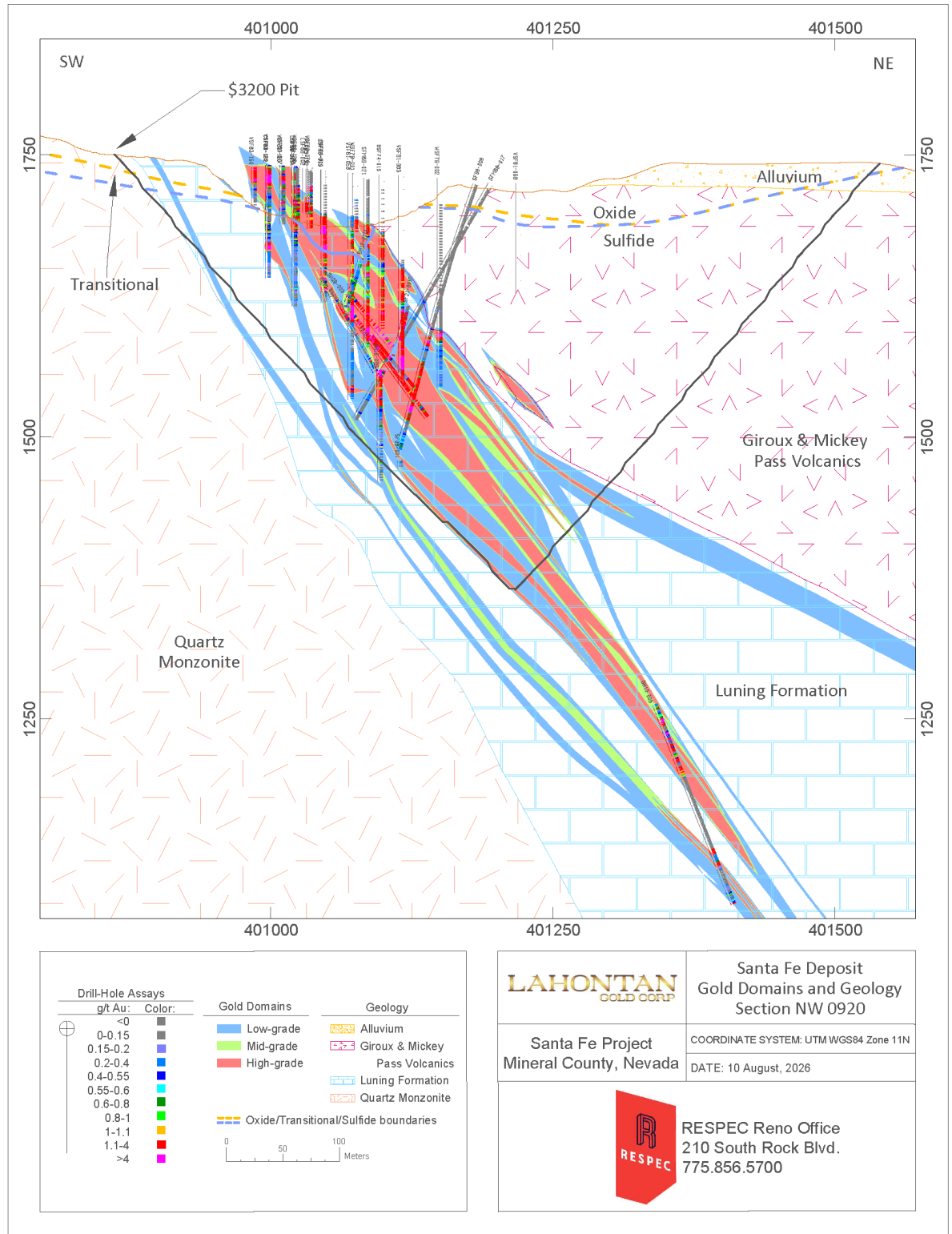
Figure 14-3. Santa Fe Deposit Gold Domains and Geology – Section NW0920 (section location on Figure 14-1)
