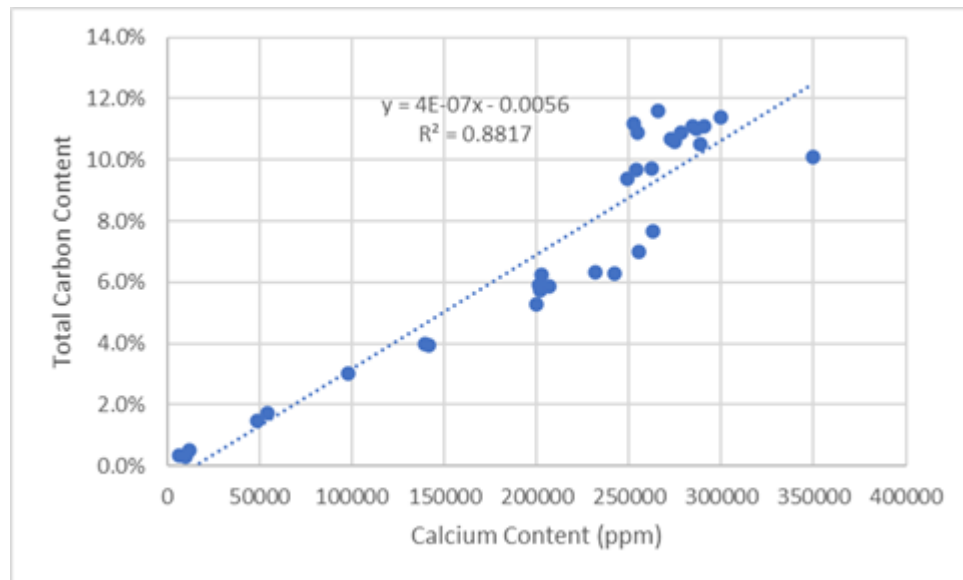
Figure 26-2. Total Carbon Content by LECO compared with Calcium Content from 2024 KCA Test Work (KCA [2024])
