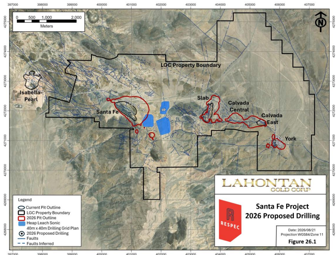
Figure 26-1. Plan Map Showing Proposed Drill Holes
