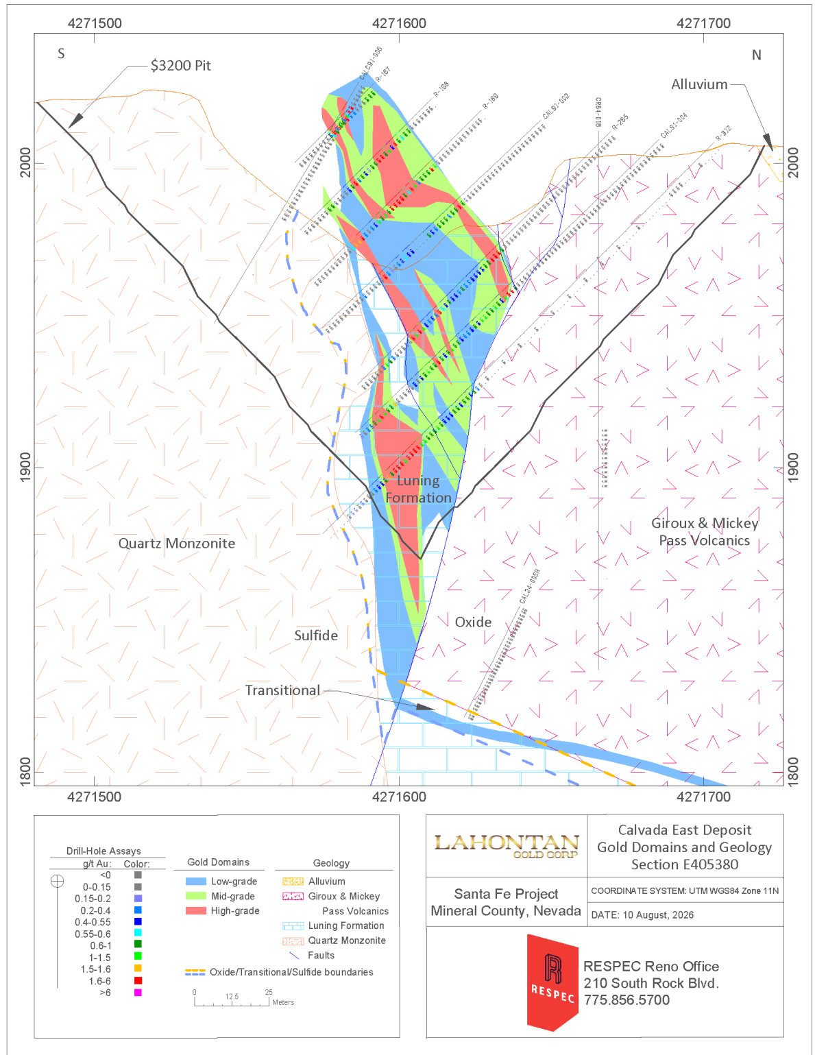
Figure 14-6. Calvada East Deposit Gold Domains and Geology – Section E405380
