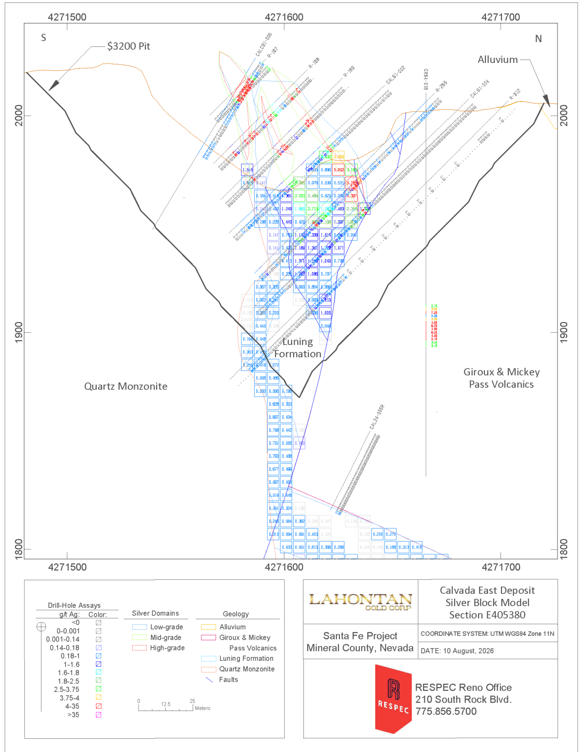
Figure 14-21. Calvada East Deposit Silver Domains and Block Model—Section E405380 (Section location on Figure 14-2)
